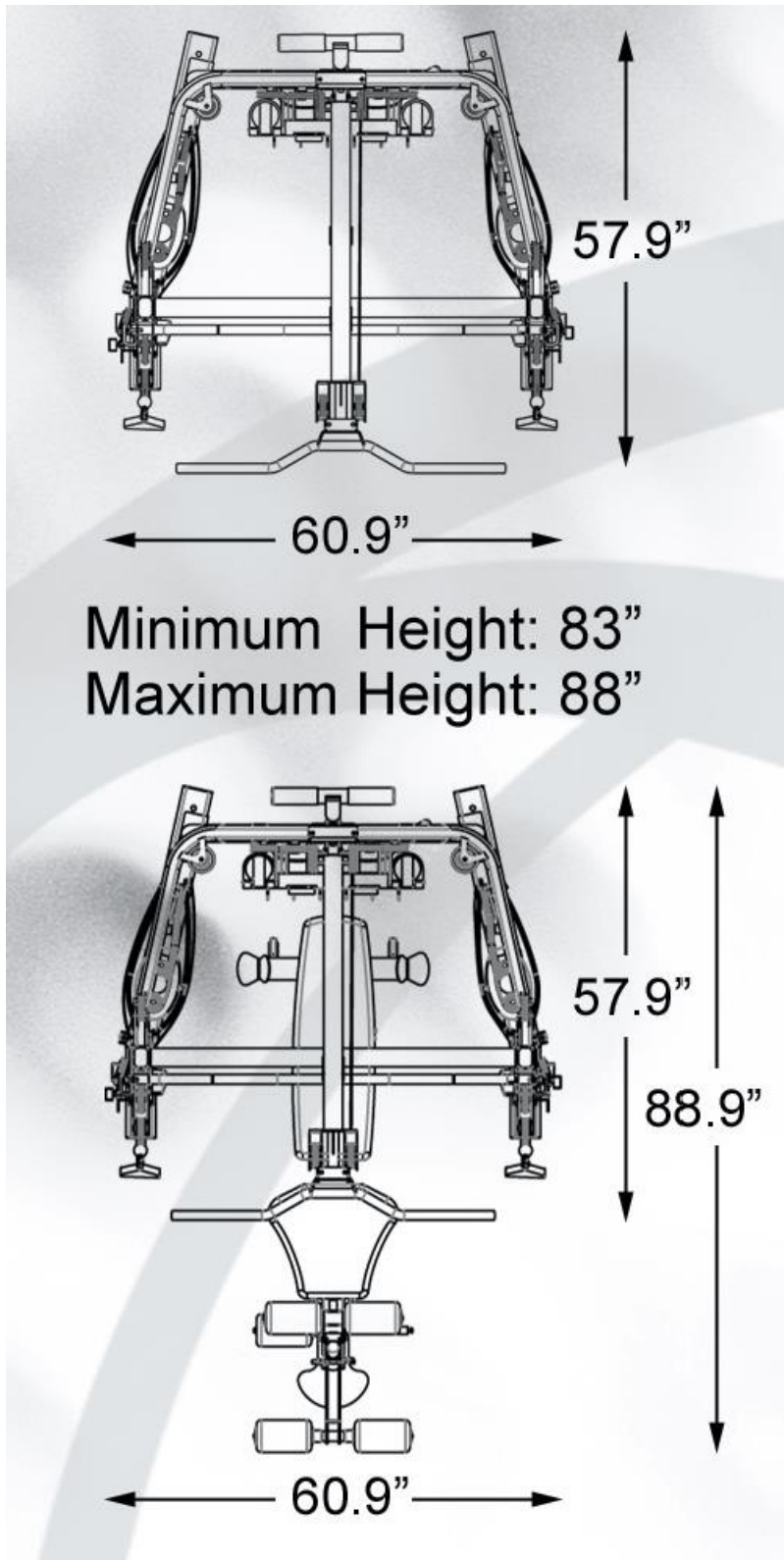
FT2 Dimensions: 61" wide x 58" deep without bench; 61" wide x 89" deep with bench; minimum height 83"; maximum height 88"
